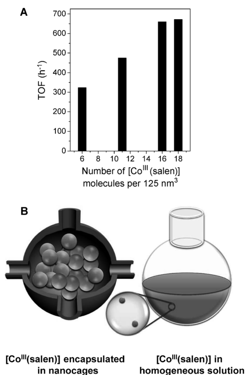
Figure 3. A) TOF of PO hydration in the presence of FDU-12-[Co III (salen)] with different numbers of [Co III (salen)] molecules in each nanocage. The reactions were performed in PO (50 mmol) with a [catalyst]/[PO]/[H 2 O] molar ratio of 1:500:1000 at 40 °C, and the TOFs were calculated for the initial 20 min. B) Illustration of the enhanced cooperative activation effect of [Co III (salen)] for the hydration of epoxides in nanocages (on average 6–18 [Co III (salen)] molecules in nanocages and 1.4 [Co III (salen)] molecules in a homogeneous solution per 125 nm 3 ).
